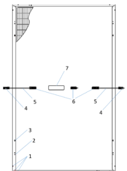
Mechanical drawing for bifacial modules
