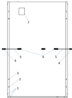
Mechanical drawing for monofacial modules
